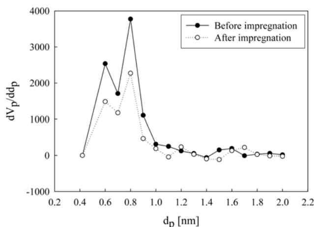
Fig. 3. Pore size distribution of C-1 before and after impregnation of 10 wt% PdCl 2 .
