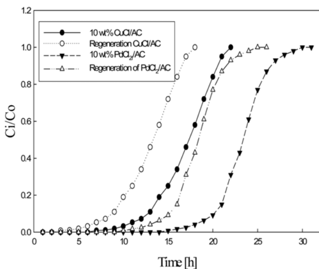
Fig. 9. Breakthrough curves in FCC C 4 feed with the spent 10 wt% CuCl/AC and the spent 10 wt% PdCl 2 /AC.
